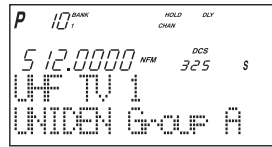
Tone SQ on, DCS 325 set
