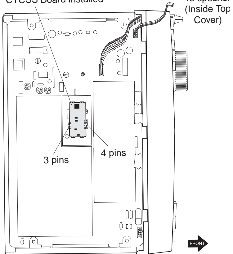
CTCSS Board installed
